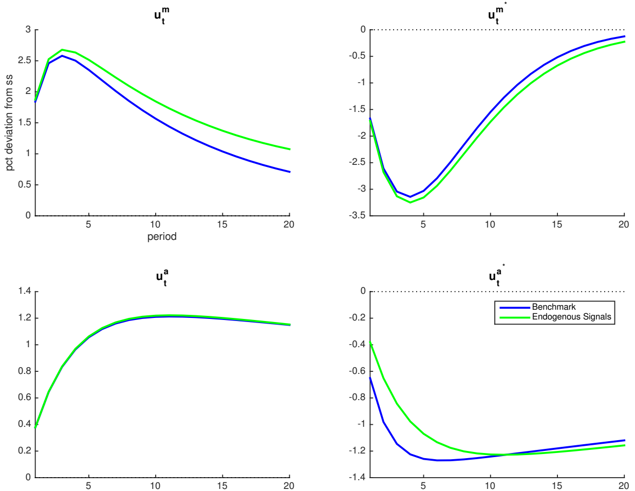
Figure 9: Impulse Response Comparison with Endogenous Signals
